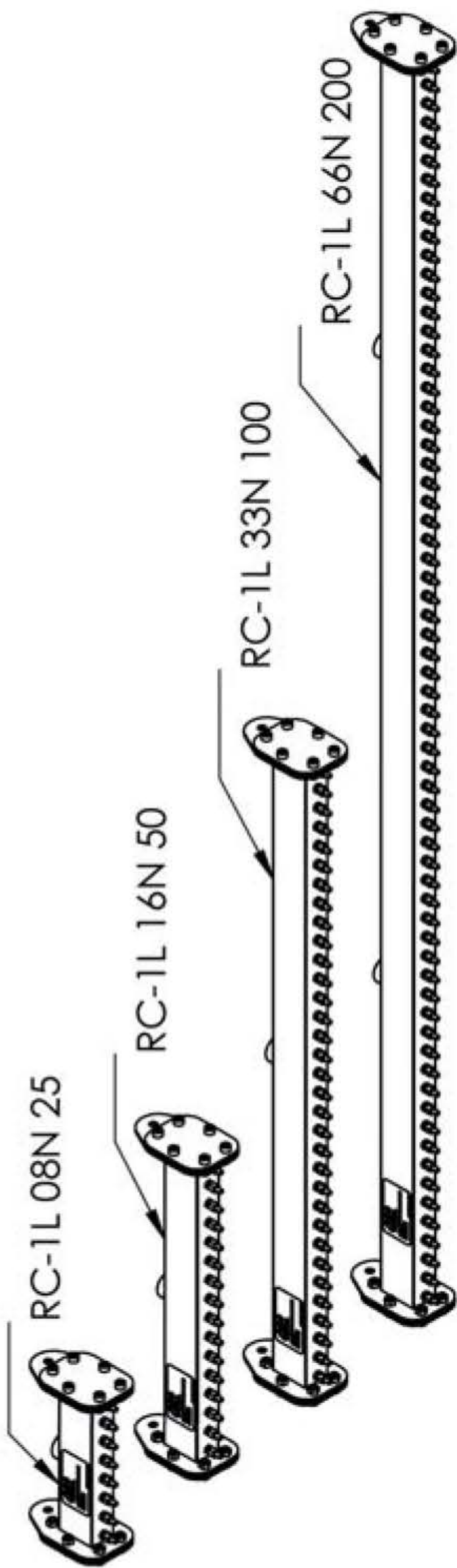
Figure 1-1 : RC1L
